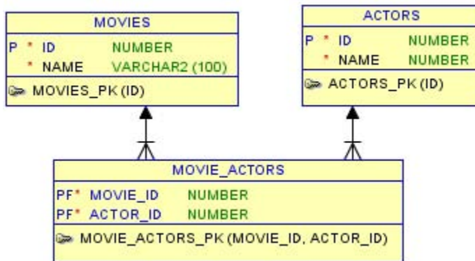
Figure 11-25. Many-to-many relationship
